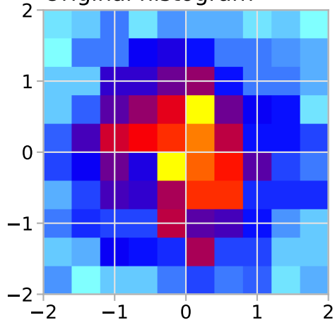
Original histogram
