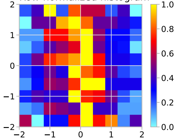
Row-normalized histogram
