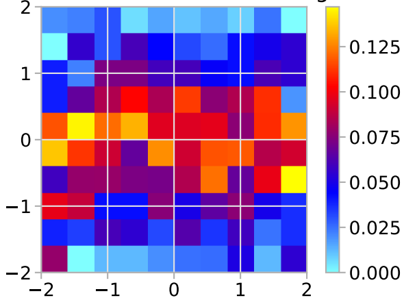
Column-normalized histogram
