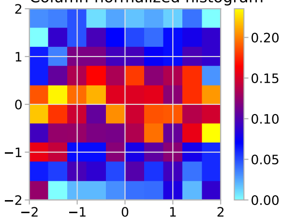
Column-normalized histogram
