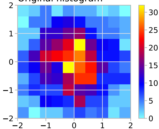
Original histogram
